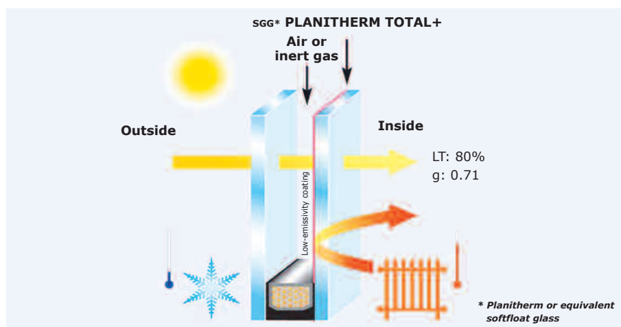
Double glazed unit with SGG PLANITHERM TOTAL+
