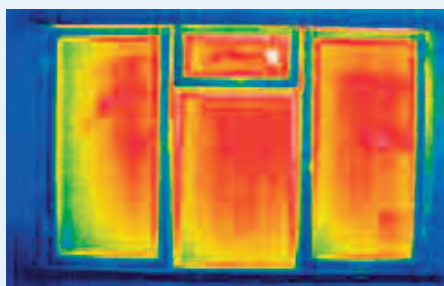
Thermal image showing heat escaping through an old wooden window
